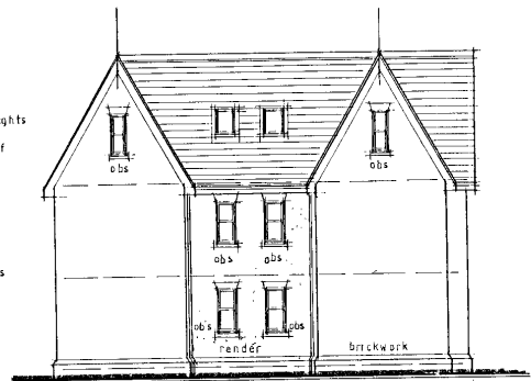
SOUTH-WEST ELEVATION
